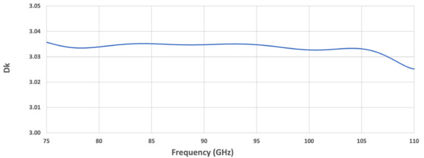
Figure 3: Dielectric constant at mmWave frequencies (WP030: Dk = 3.03 @ 5 GHz)
