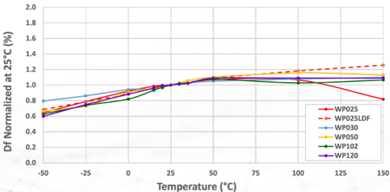
Figure 2: Thermal Coefficient of Loss Tangent
