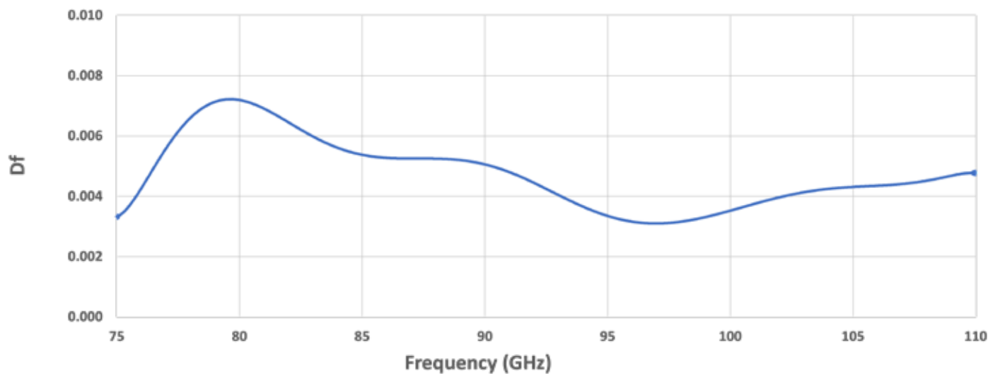
Figure 4: Loss tangent at mmWave frequencies (WP030: Df = 0.0009 @ 5GHz)
