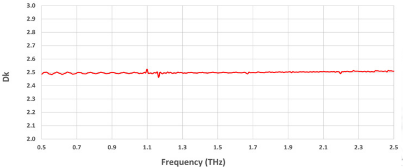
Figure 5: Dielectric constant at Terahertz frequencies WP025: Dk = 2.5 @ 5 GHz
