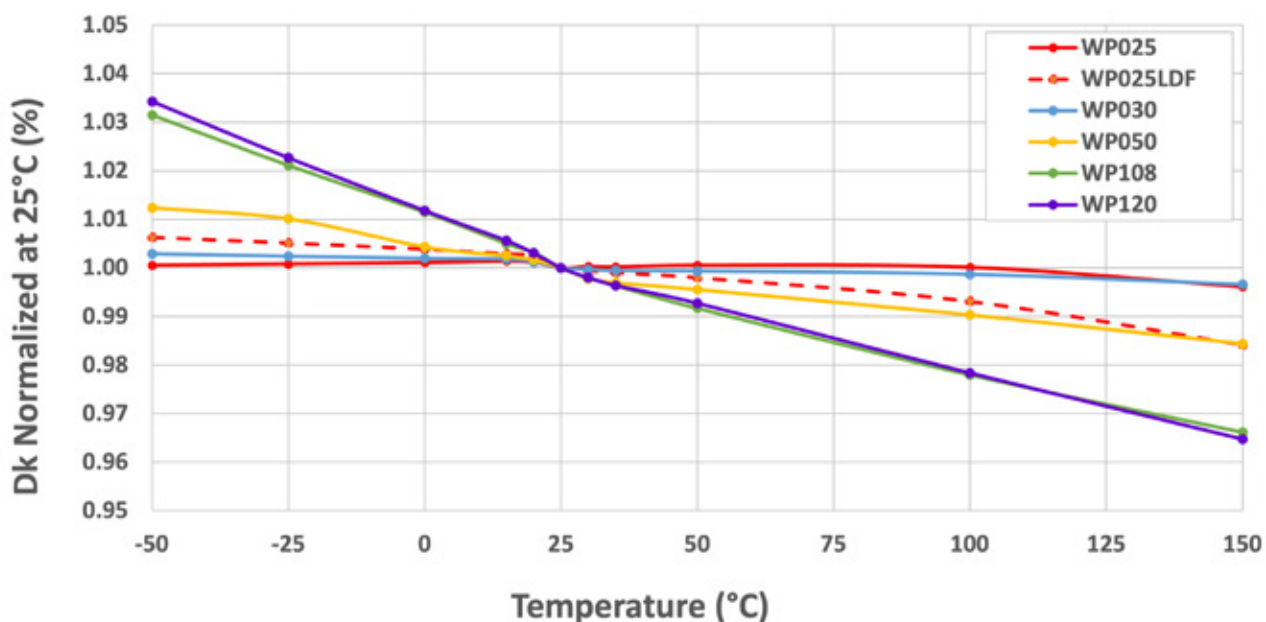
Figure 1: Variation of Dielectric Constant Dk with Temperature
